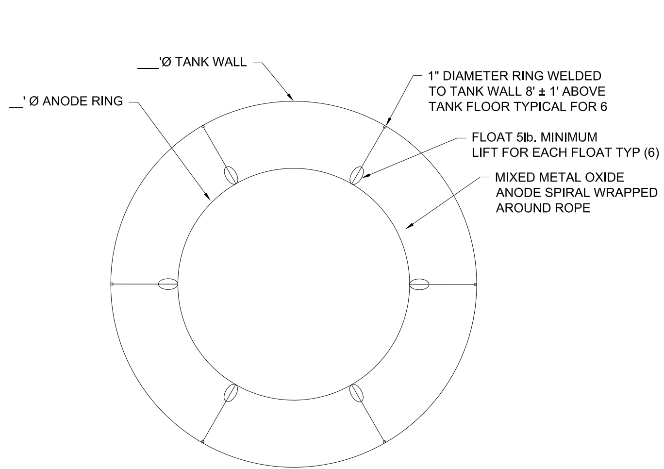
TYPICAL FLOATING OR SUBMERGED ANODE LAYOUT
